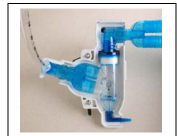
The Swirler UltraShield® is injection molded of a Tungsten formulation to conform to the shape of the Swirler Aerosol System. This new material and process makes the combination light in weight while maintaining desirable Lead equivalent shielding.
